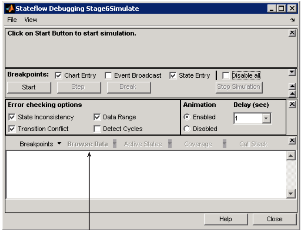
Menu for observing data when simulation pauses at a breakpoint
